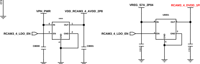
RCAM3_4_AVDD
