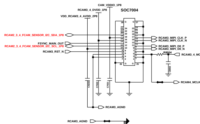
RCAM3_2M_BOKEH (24PIN)_GC02M1B COPY FROM SM-A13_LTE
